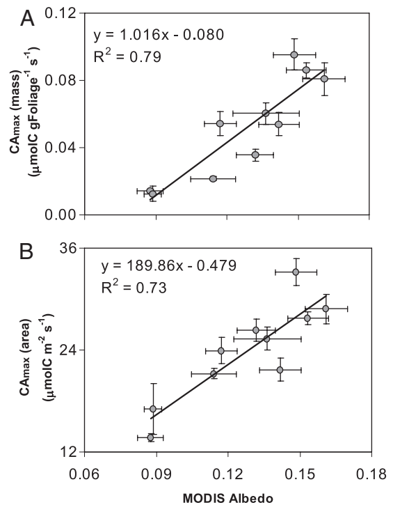
Fig. 3. Shortwave growing season albedo from the MODIS instrument in relation to (A) C_{A_{max}} expressed per unit of canopy leaf mass and (B) C_{A_{max}} expressed per unit of ground area. Albedo uncertainty terms are standard deviations of all growing season observations between 2000 and 2006.
